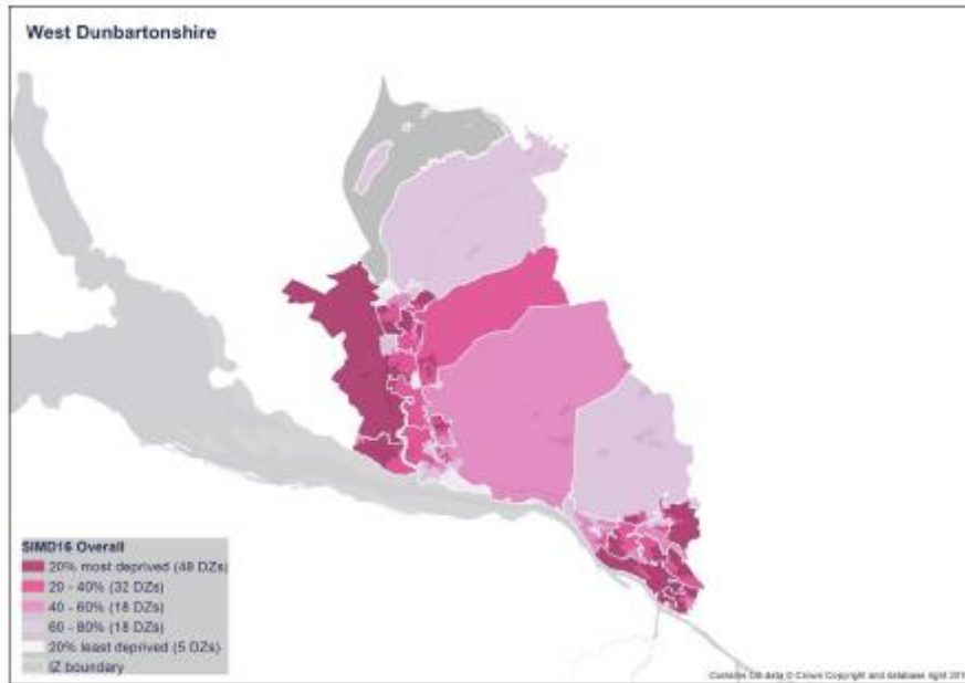
SIMD16 quintiles
