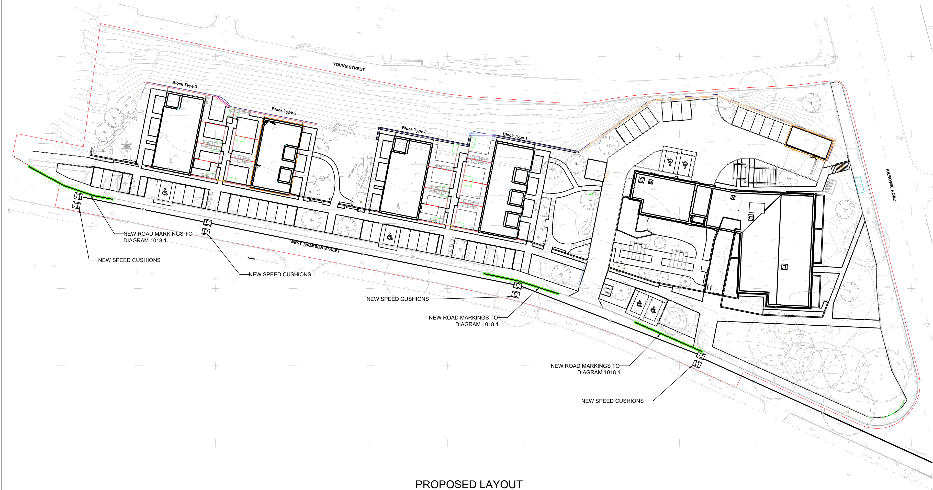
PROPOSED LAYOUT (Scale 1:100)
